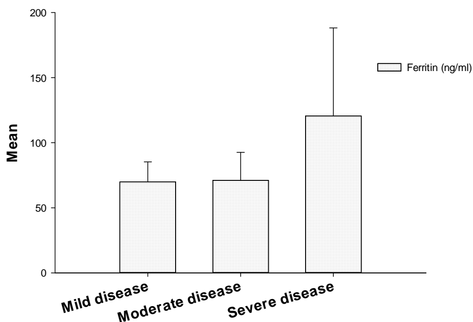
Fig. 1. Bar chart showing degrees of disease severity against mean serum ferritin levels in SCD subjects
